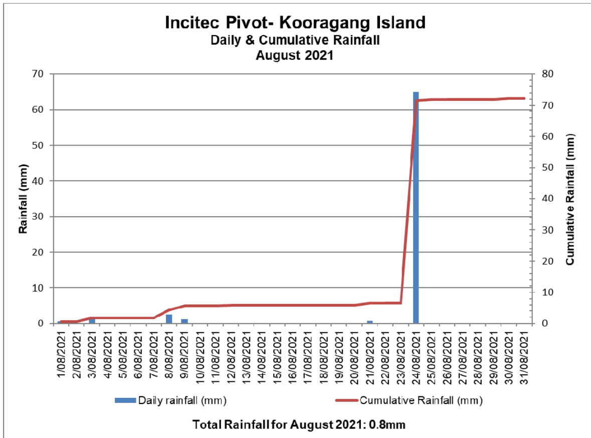
Figure 1 August 2021 Rainfall Summary
